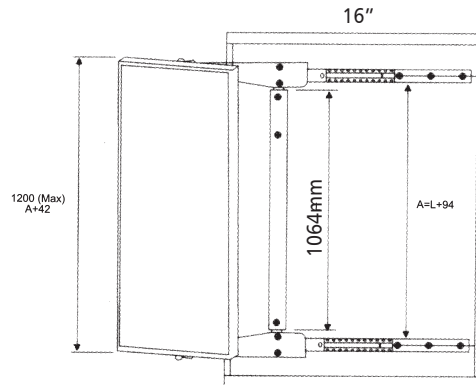
2704 Extension Mirror Guide for Wardrobe 16" Black Length of Bar - 1064mm
