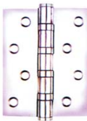
Stainless Steel Hinge 2" x 1.2mm 2.5" x 1.2mm 3" x 1.5mm 4" x 3" x 2mm 4" x 3" x 3mm 5" x 3.5" x 3mm
