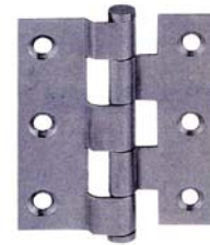
Aluminium Frame Door Hinge 4"x3"x2.0mm 304 Stainless Steel
