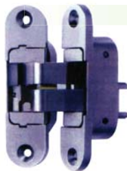
ST-C118 Suitable for doors from 600 to 1000mm width and up to 2700mm height with a minimal door thickness of 40mm. Load capacity 80kgs. *We recommend always 3 hinges installed!
