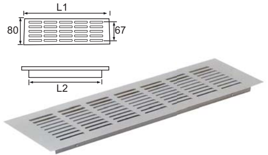
WH-01 L1: 150, 250, 300, 400, 450mm Aluminium Ventilator
